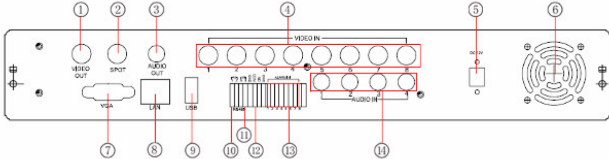
Fig 2.7 Rear Panel for 8-ch
