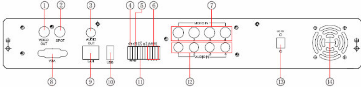
Fig 2.6 Rear Panel for 4-ch
